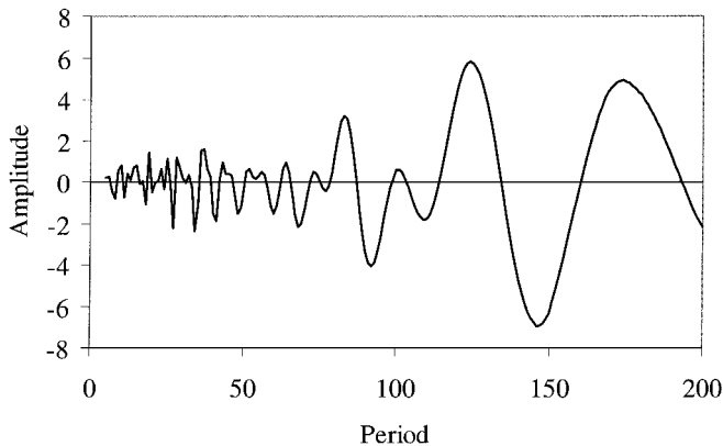
FIG. 4. Cosine spectrum of eukaryotic enzyme lengths, entire data set. The cosine spectrum generated by SAD achieves a maximum amplitude at 124 aa.
