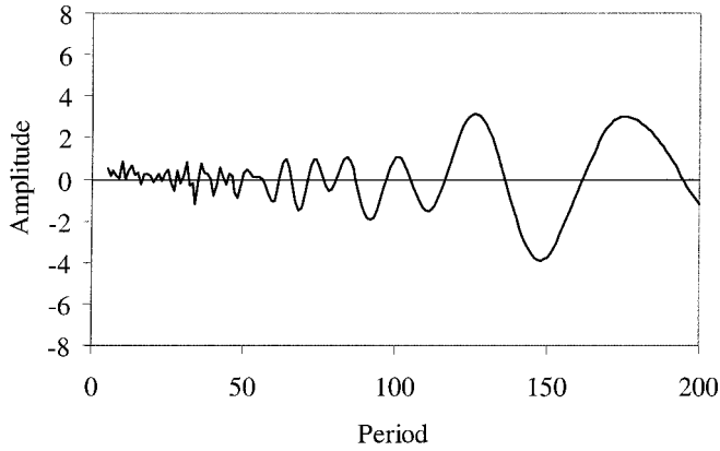
FIG. 6. Cosine spectrum of eukaryotic enzyme lengths, non-redundant data set. The cosine spectrum generated by SAD achieves a maximum amplitude at 126 aa.
