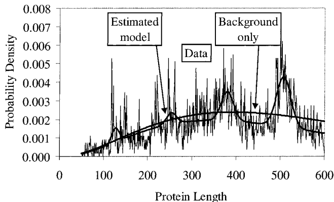
FIG. 7. Estimated probability density of eukaryotic enzyme lengths, nonredundant data set. The data are shown with the estimated model and the constrained model consisting of background only without any peaks.
