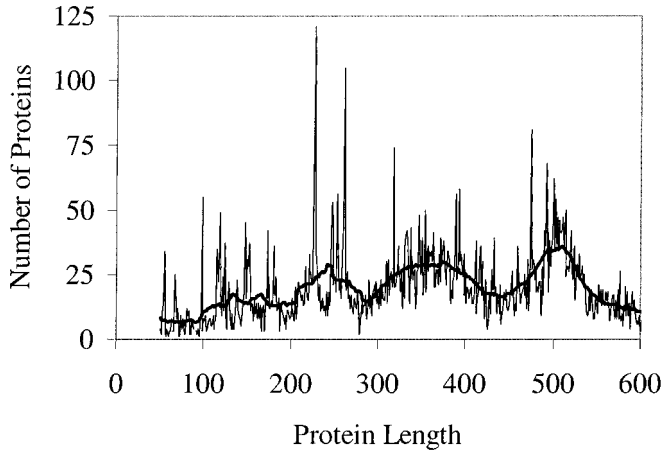
FIG. 1. Distribution of eukaryotic enzyme lengths, entire data set. The histogram corresponds to the actual (raw) distribution, and the smoothed curve corresponds to the running averages with a 41-aa window.
