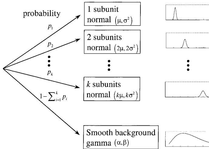
FIG. 2. Mixture distribution model. The model consists of a smooth background together with superimposed peaks in the distribution.
