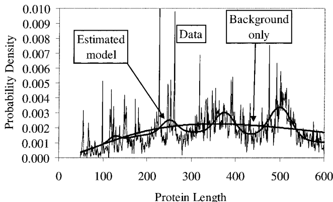
FIG. 3. Estimated probability density of eukaryotic enzyme lengths, entire data set. The data are shown with the estimated model and the constrained model consisting of background only without any peaks.
