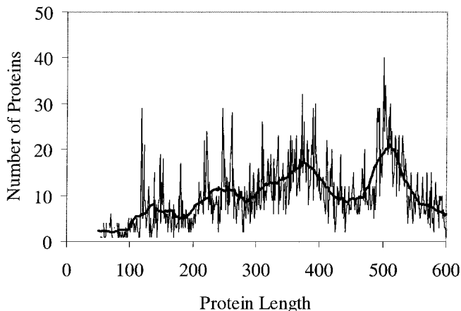
FIG. 5. Distribution of eukaryotic enzyme lengths, nonredundant data set. The histogram corresponds to the actual (raw) distribution, and the smoothed curve corresponds to the running averages with a 41-aa window.
